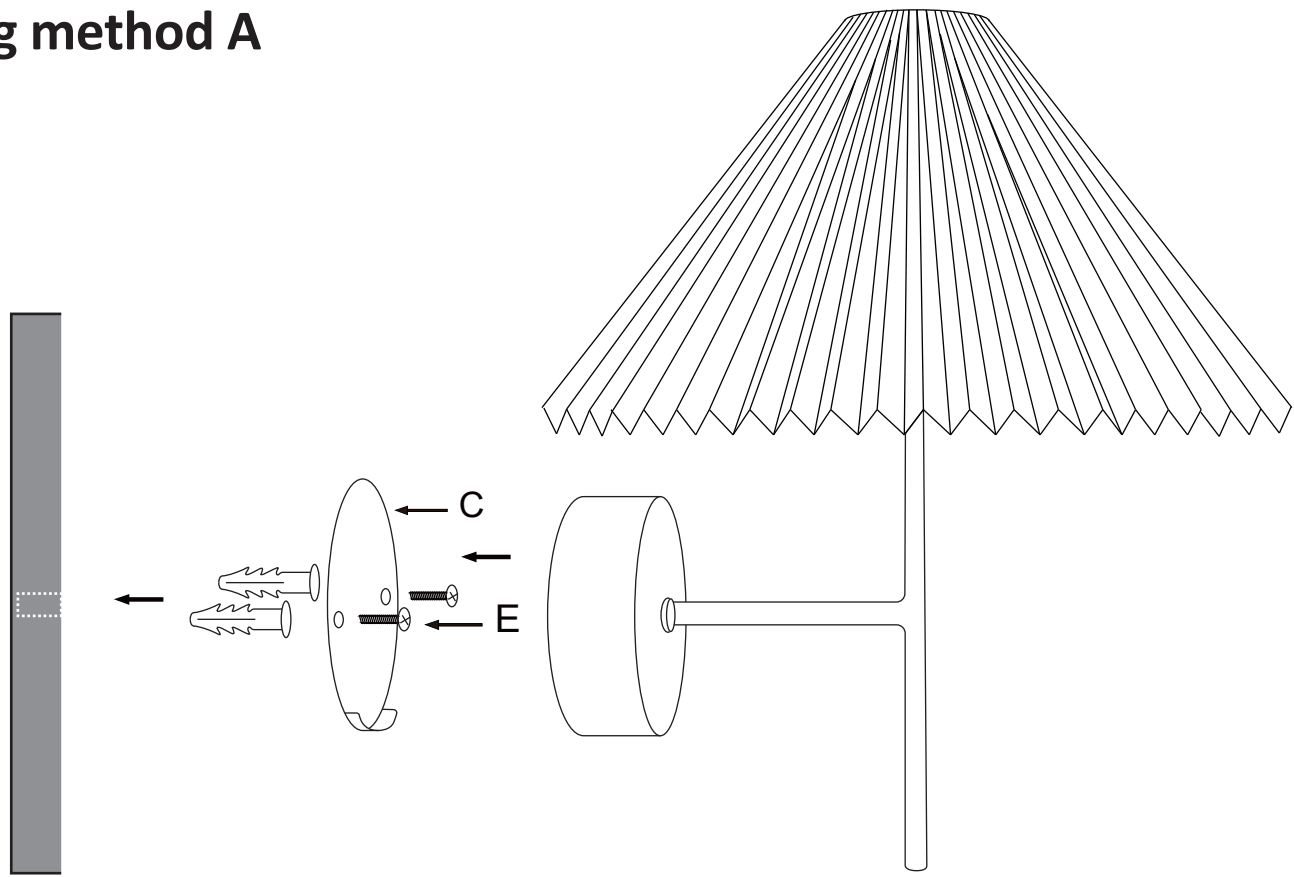
Fix the lamp on the wall with screws.
