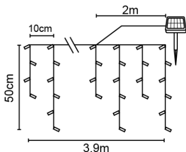
Assembly Diagram:
