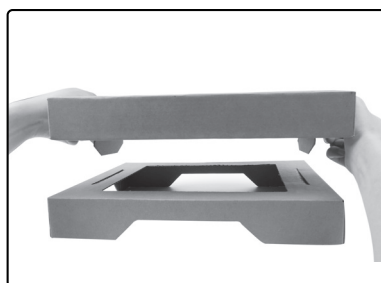
Setp 3: Insert the brazier into the base.
