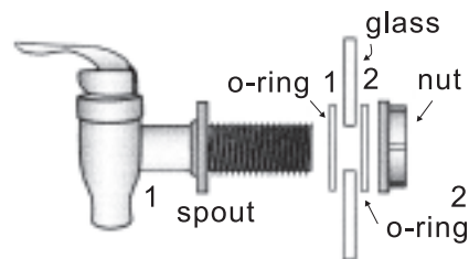
Expanded view of parts supplied
