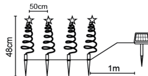
Assembly Diagram:
